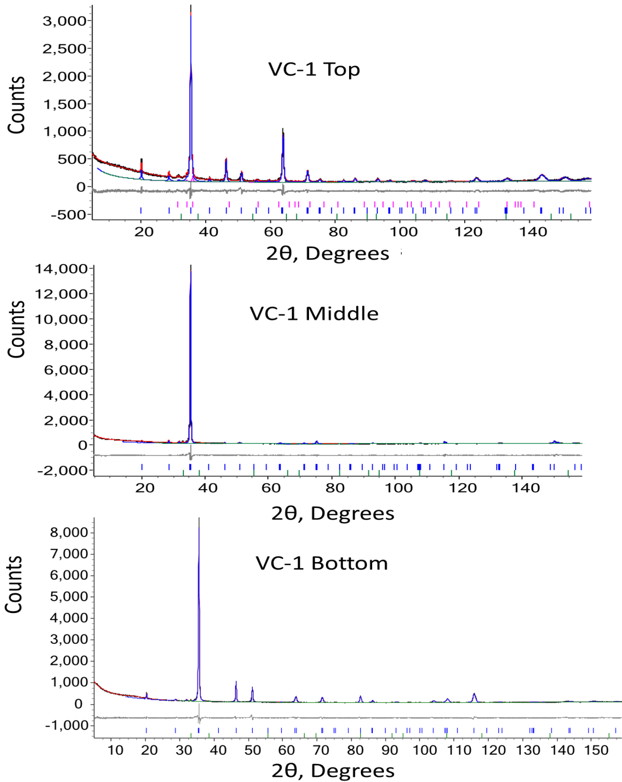
Figure 4: XRD results from VC-1 Top, Middle, and Bottom sections is shown by the black line. The delta phase, \text{UZr}_2 , is fit with a blue line, \text{ZrC} with green, and \alpha\text{-Zr} with pink. The overall fit is in red and the difference between fit and observed data is in grey.
