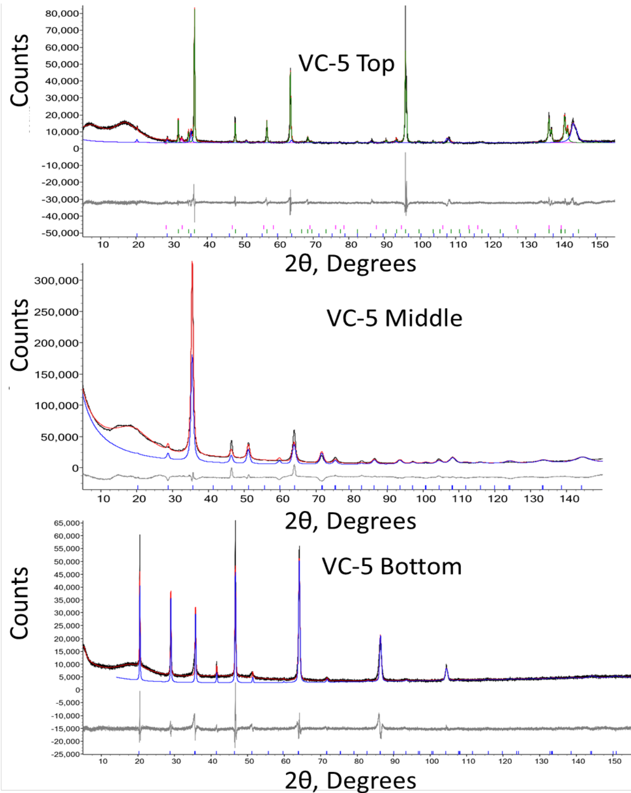
Figure 19: XRD results from VC-5 top and bottom samples are shown by the black line. The delta phase, \text{UZr}_2 , is fit with a blue line, \alpha -Zr with a green line and \text{UO}_2 with a pink line. The overall fit is in red and the difference between fit and observed data is in grey.
