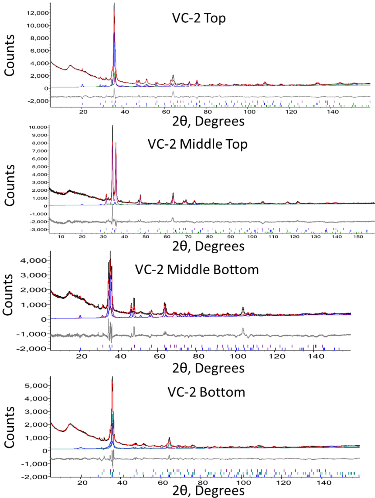
Figure 8: XRD results from VC-2 samples are shown by the black line. The delta phase, Uzr_2 , is fit with a blue line, \alpha -Zr with green, and \alpha -U metal with green. The overall fit is in red and the difference between fit and observed data is in grey.
