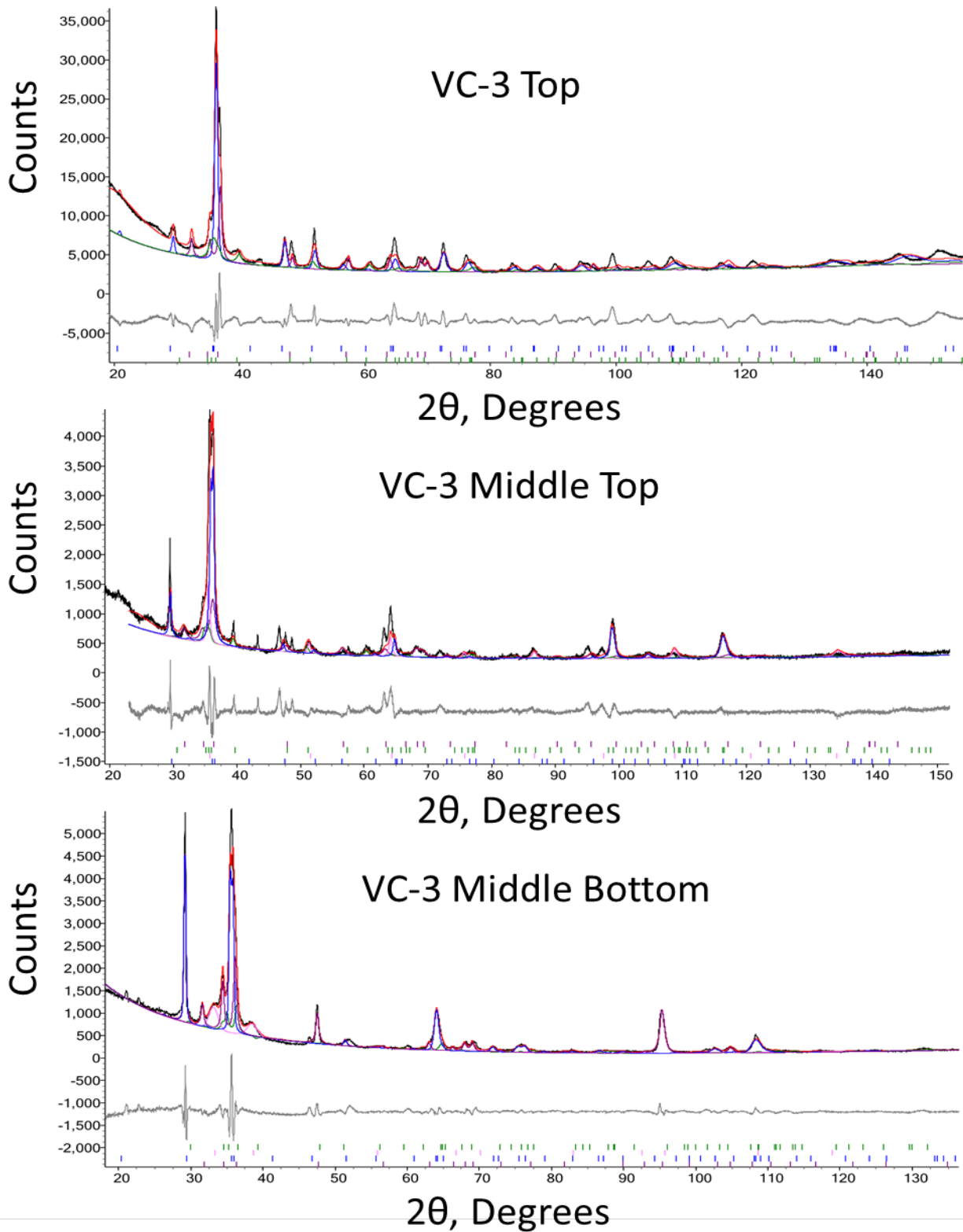
Figure 11: XRD results from VC-3 samples are shown by the black line. The delta phase, UZr_2 , is fit with a blue line, \alpha -Zr with purple, \alpha -U with green, and ZrC with pink. The overall fit is in red and the difference between fit and observed data is in grey.
