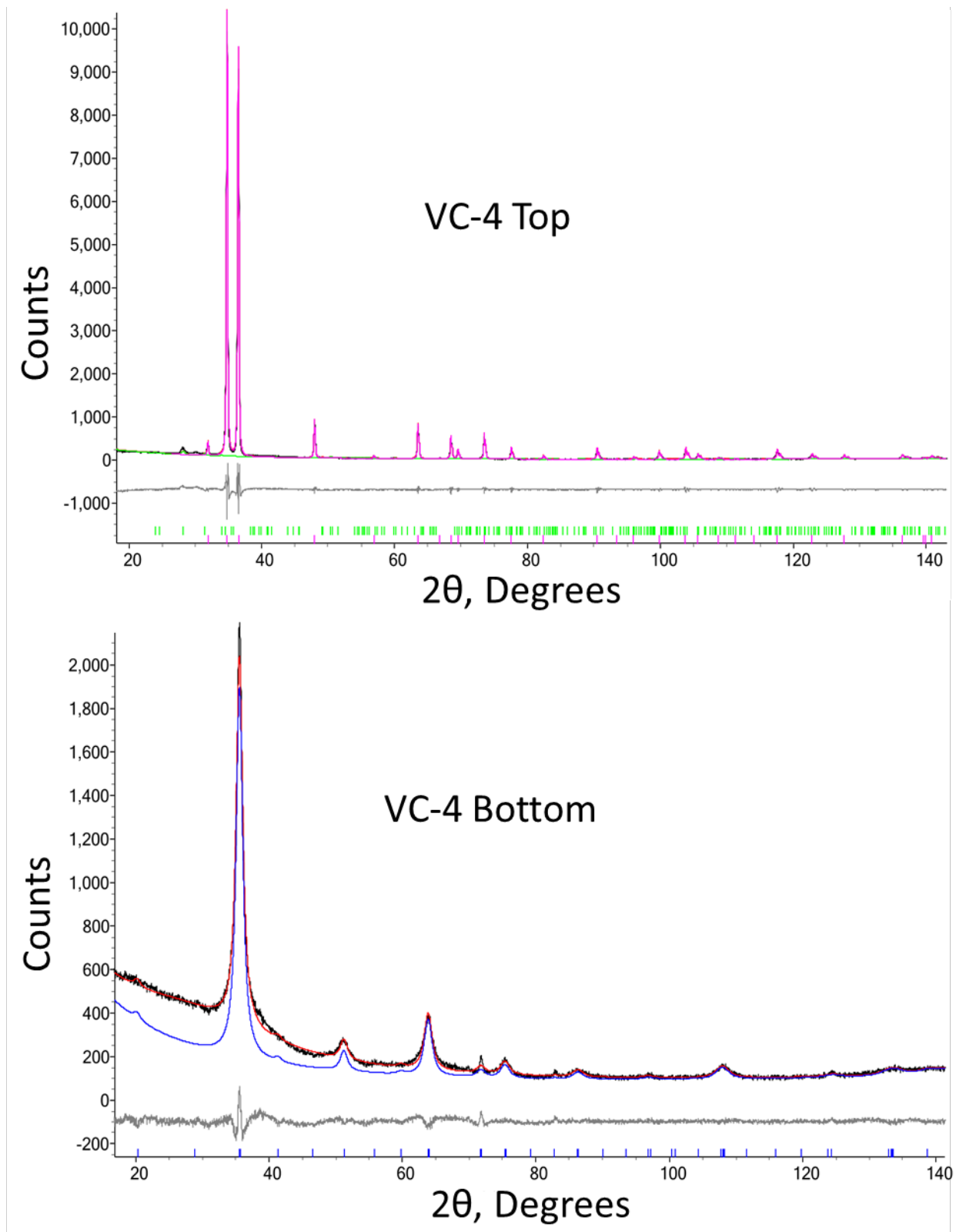
Figure 15: XRD results from VC-4 top and bottom samples are shown by the black line. The delta phase, \text{UZr}_2 , is fit with a blue line, and \alpha\text{-Zr} with a pink line. The overall fit is in red and the difference between fit and observed data is in grey.
