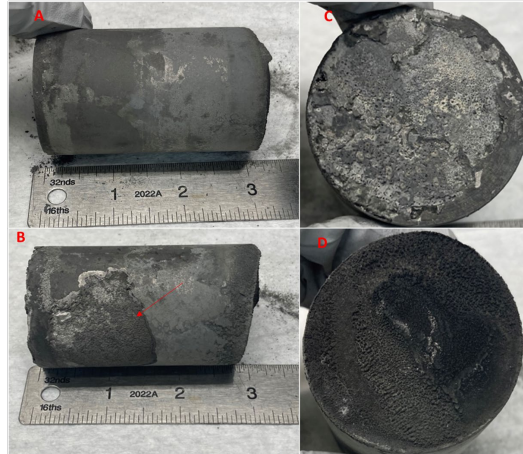
Figure 2: VC-1 billet before cleaning. A) The billet side view. B) The opposite side view with an arrow indicating where the crucible and melt reacted. C) The billet bottom contacting the crucible bottom. D) The billet top which was exposed to the VIM environment.
